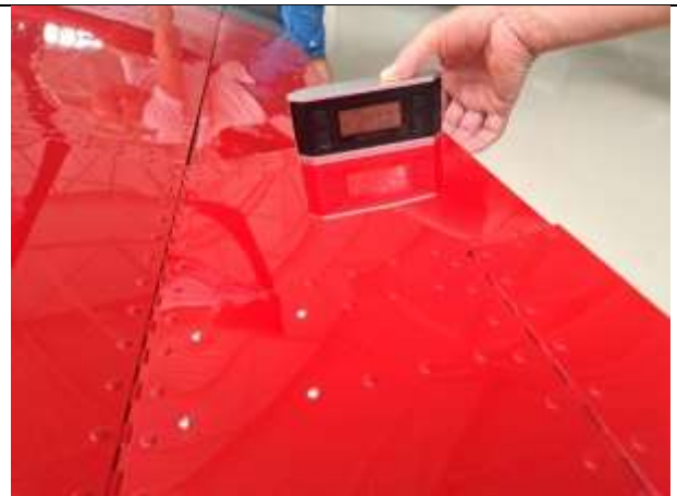
Fig. 6-10 Measure and record left aileron up deflection
