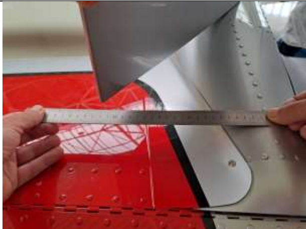
Fig. 6-20 Rudder left deflection. 30° = 225 mm
